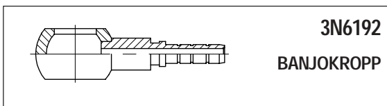
Artikel nr Beteckning 3N6192-08-03 BANJO 8MM 1/8" 3N6192-10-03 BANJO 10MM 1/8" 3N6192-10-04 BANJO 10MM 3/16" 3N6192-11-03 BANJO 11MM 1/8" 3N6192-12-03 BANJO 12MM 1/8"
