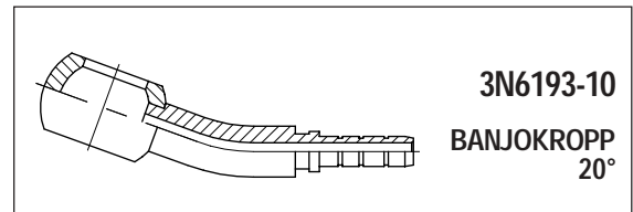
Artikel nr Beteckning 3N6193-10-03 BANJO 10MM 20° 1/8" 3N6193-10-04 BANJO 10MM 20° 3/16" 3N6193-11-03 BANJO 11MM 20° 1/8"
